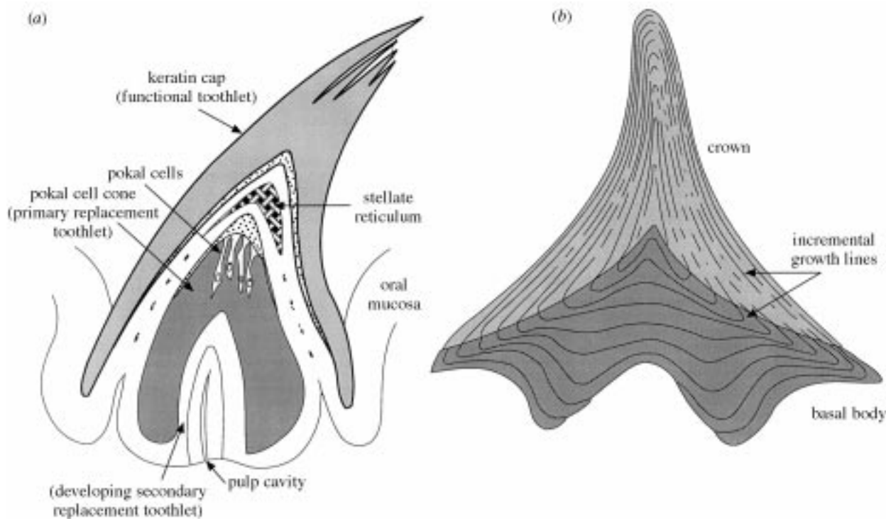
Figure 2. (a) Lingual tooth of Myxine Linnaeus in longitudinal section, after Dawson (1963) and Kresja (1990 a,b ). (b) Pa element of Ozarkodina in transverse section, after Müller & Nogami (1971). The functional keratin cap and replacement toothlet (pokal cell cone) of the myxinoid grow as distinct structures, whereas the crown and basal body (putative replacement crown of Kresja (1990 a,b )) grow in intimate association.
