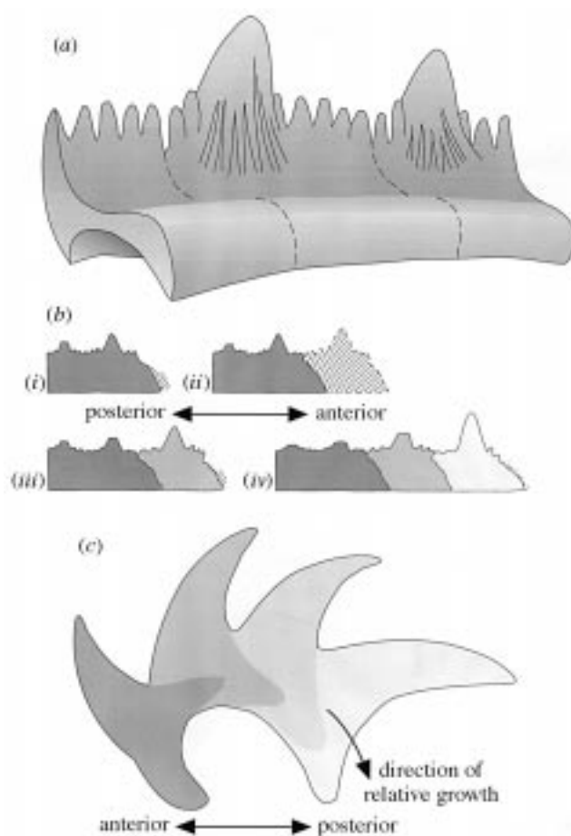
Figure 15. (a) Part of a dentigerous jaw bone in Xylacanthus grandis Ørvig, after Ørvig (1967 b , 1973) with omission of the supporting jaw cartilage. Dashed lines delineate units of growth. (b (i)–b(iv) ) Illustration of growth of acanthodian dentigerous jaw bone by marginal accretion at the anterior end of the jaw. Illustration also includes successive wearing-down of the teeth, after Ørvig (1973). (c) Illustration of growth of acanthodian tooth whorl, based on Nostolepis Pander. Shading delineates units of growth that were added to the posterior of the whorl, after Ørvig (1973).
